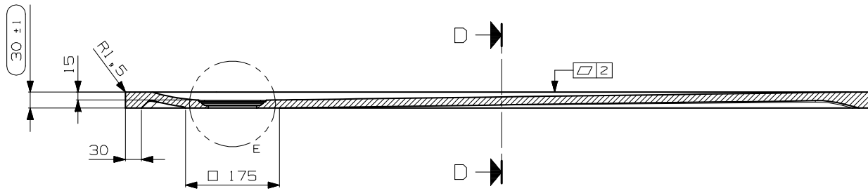
SECTION C-C SCALE 0.143:1.0
